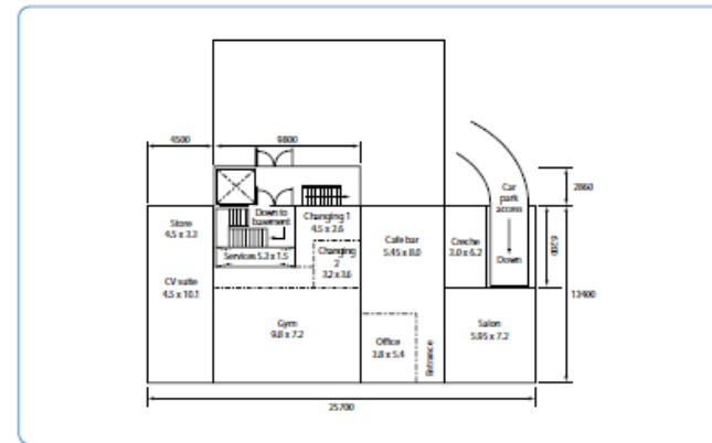
Figure 3: General Arrangement - Ground Floor Plan
