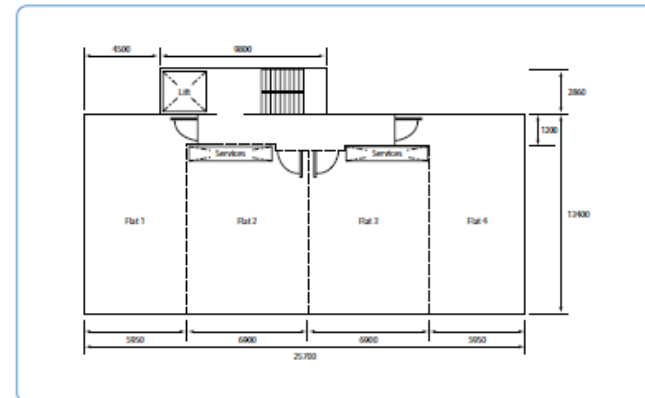
Figure 4: General Arrangement - Typical Residential Floor Plan
