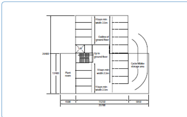
Figure 2: General Arrangement Basement Level
